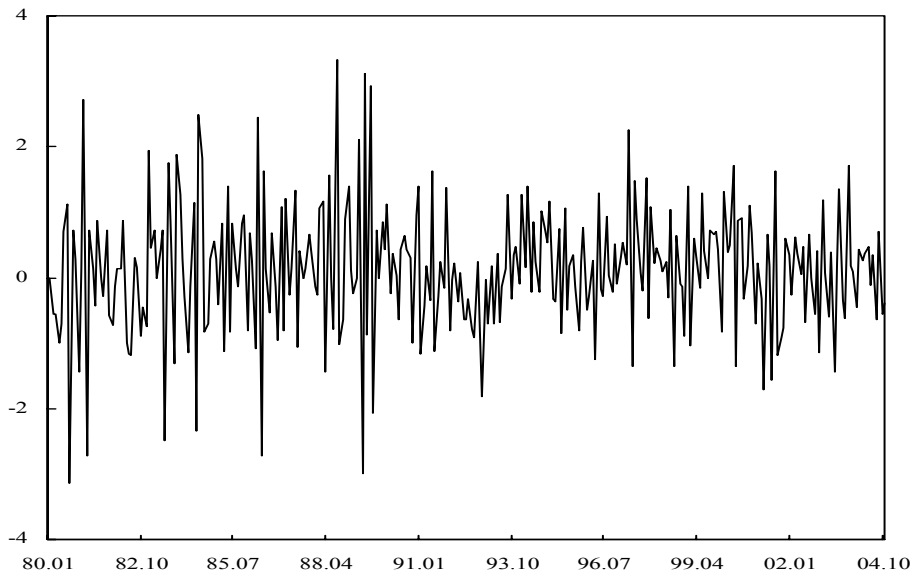
Figure 3: Monthly growth rates of IPI, 80.01-04.11.
