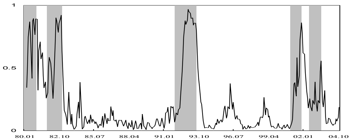
Figure 4: Filtered probabilities of recessions from univariate Markov-switching model applied to IPI. Shaded areas represent classical recessions obtained by applying Bry-Boschan to IPI. Sample: 80.01-04.11.
