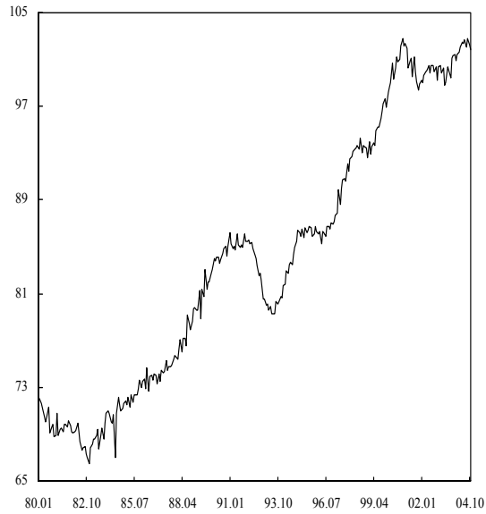
Figure 1: Euro-area Industrial Production Index (IPI), 80.01-04.11.
